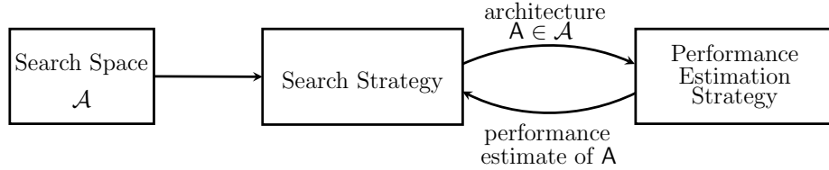
Figure 3.1: Abstract illustration of Neural Architecture Search methods. A search strategy selects an architecture A from a predefined search space \mathcal{A} . The architecture is passed to a performance estimation strategy, which returns the estimated performance of A to the search strategy.
